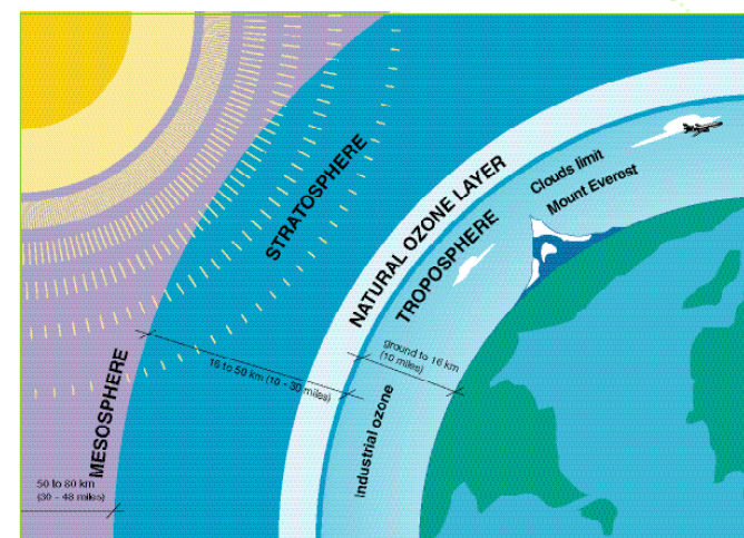
illustration 3 : THE OZONE LAYER BETWEEN THE SUN AND THE EARTH
