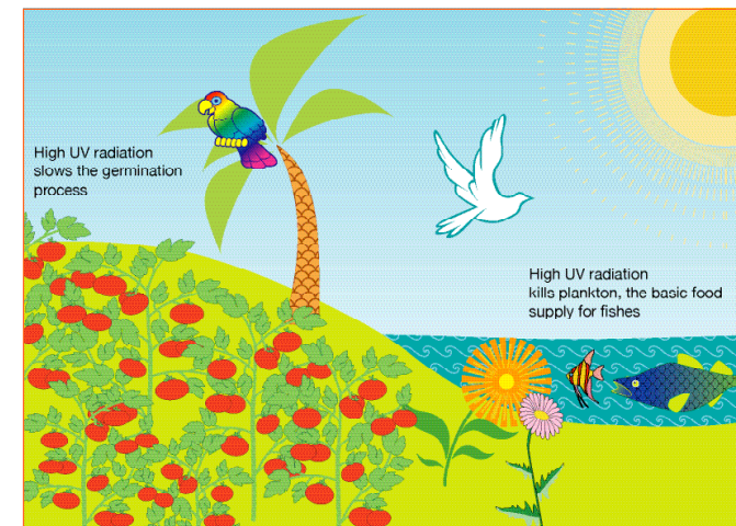
Illustration 11 : HIGH UV RADIATION AND THE ENVIRONMENT
