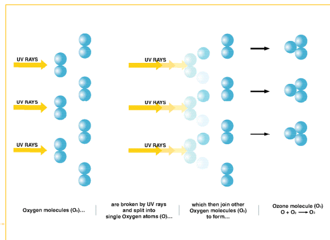
Illustration 5: FORMATION OF NATURAL OZONE
