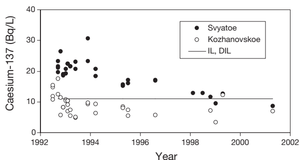
FIG. 3.49. Dynamics of ^{137}\text{Cs} activity concentration in the water of Lakes Svyatoye and Kozhanovskoye (Russian Federation), approximately 200 km from Chernobyl [3.118].
