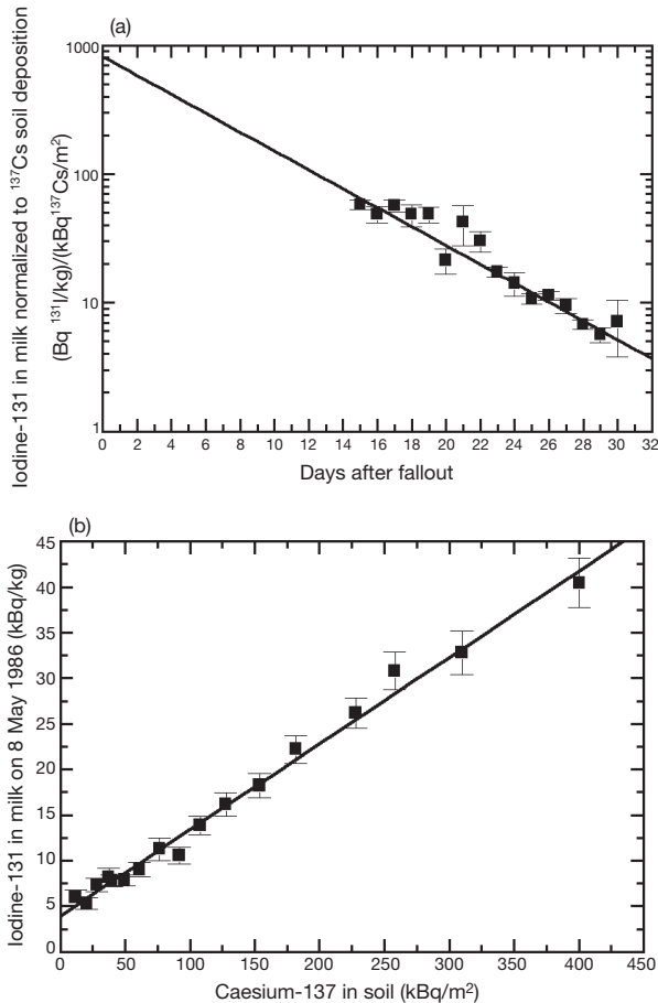
FIG. 3.14. Variation in ^{131}\text{I} activity concentration in milk in the Tula region of the Russian Federation (a) with time after deposition, standardized by ^{137}\text{Cs} soil deposition, and (b) with ^{137}\text{Cs} soil deposition (time corrected to 8 May 1986) [3.30].
