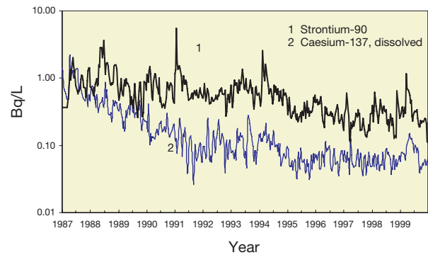
FIG. 3.45. Monthly averaged ^{90}\text{Sr} and ^{137}\text{Cs} activity concentrations in the Pripyat River near Chernobyl [3.106].
