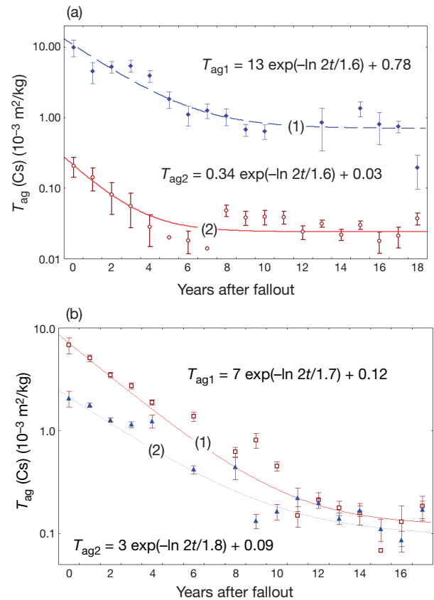
FIG. 3.30. (a) Dynamics of the ^{137}\text{Cs} aggregated TF for cow's milk. 1: peat bog soil, Bryansk region, Russian Federation; 2: chernozem soil, Tula and Orel regions, Russian Federation [3.56]. (b) Dynamics of ^{137}\text{Cs} aggregated TF for cow's milk (sandy and sandy loam soil, Bryansk region, Russian Federation). 1: ^{137}\text{Cs} soil deposition <370 kBq/m 2 ; 2: ^{137}\text{Cs} soil deposition >370 kBq/m 2 [3.56].
