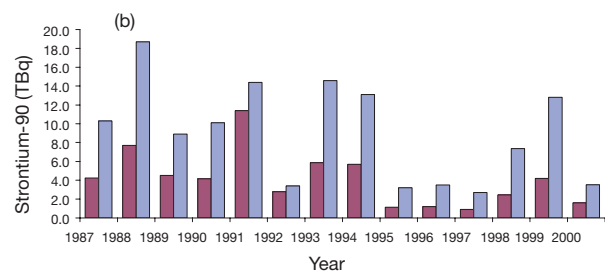
FIG. 3.46. Annual fluxes of ^{137}\text{Cs} (a) and ^{90}\text{Sr} (b) in the Pripyat River at Belaya Soroka, near the Belarus–Ukraine border (inlet to the CEZ), and downstream of Chernobyl (outlet of the CEZ) [3.107].
