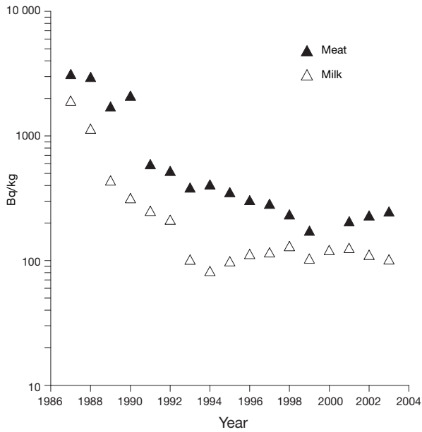
FIG. 3.29. Changes with time in mean ^{137}\text{Cs} activity concentrations in meat and milk produced in contaminated districts of the Bryansk region of the Russian Federation (Bq/kg) [3.55].
