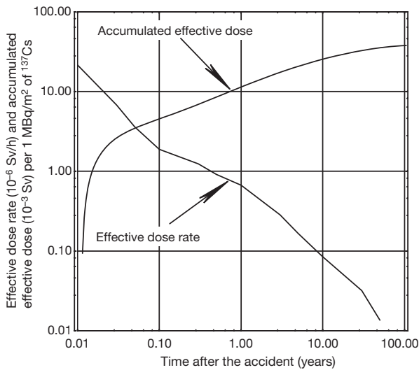
FIG. 5.8. Model prediction of the time dependence of the external effective gamma dose rate and the accumulated external effective dose to the urban population of the Bryansk region of the Russian Federation [5.7].
