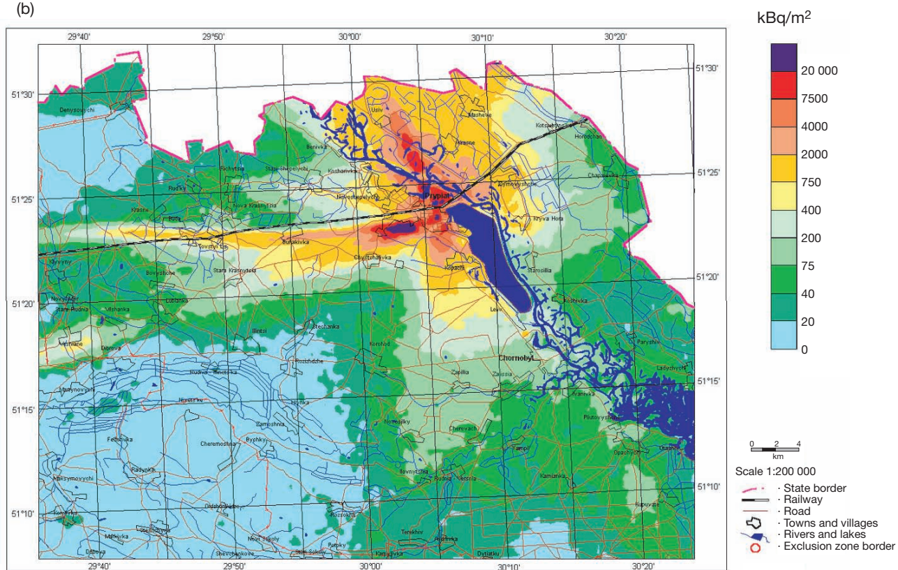
FIG. 7.6. Surface contamination by radioactive fallout within the CEZ [7.2]. (a) Caesium-137 in soils of the CEZ in 1997 (kBq/m 2 ); (b) ^{90}\text{Sr} in soils of the CEZ in 1997 (kBq/m 2 ); (c) ^{241}\text{Am} in soils of the CEZ in 2000 (kBq/m 2 ); (d) ^{239,240}\text{Pu} in soils of the CEZ in 2000 (kBq/m 2 ).
