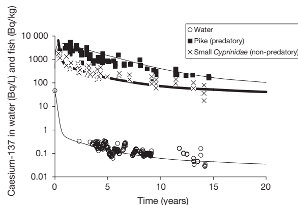
FIG. 3.48. Time series of ^{137}\text{Cs} in Lake Vorse, Germany [3.93].
