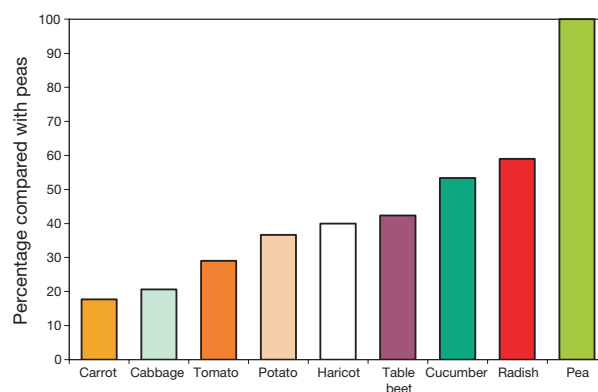
FIG. 4.6. Comparison of ^{137}\text{Cs} uptake in different crops, normalized to that of peas [4.39].
