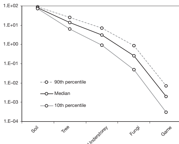
FIG. 3.36. Calculated percentage distributions of radiocaesium in specified components of coniferous forest ecosystems [3.73].
