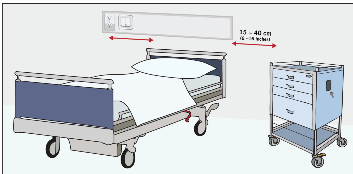
Figure 2.2 Appropriate workspace and reach distance for workers at the bedside
