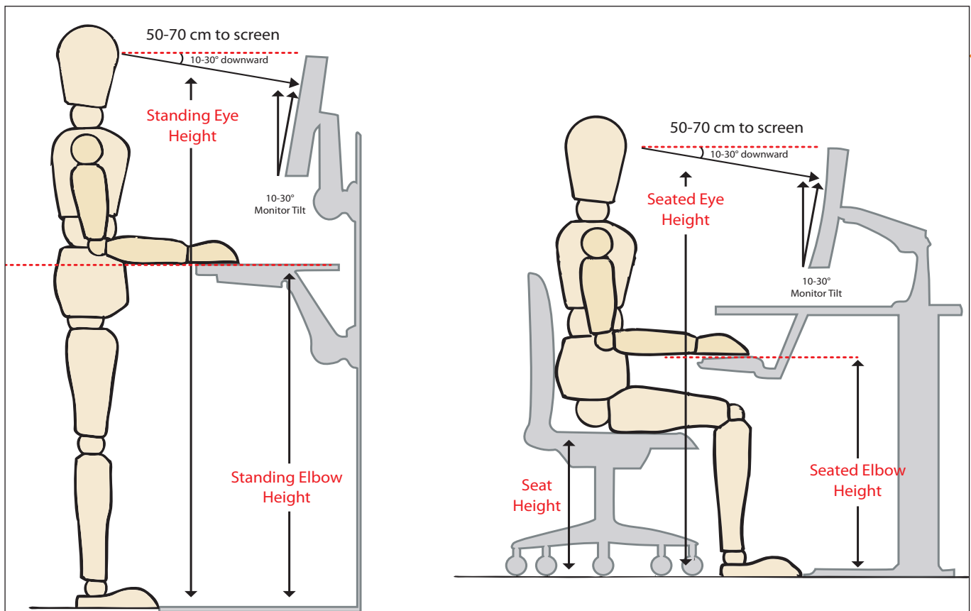
Figure 2.3 Recommended dimension for standing and seated tasks
